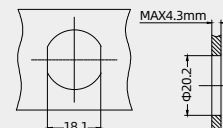
Panel Cut-out
